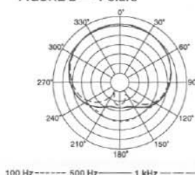
FIGURE 2 — Polars
