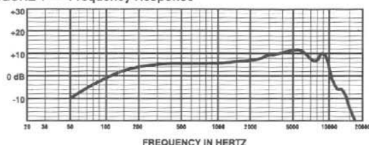
FIGURE 1 — Frequency Response
